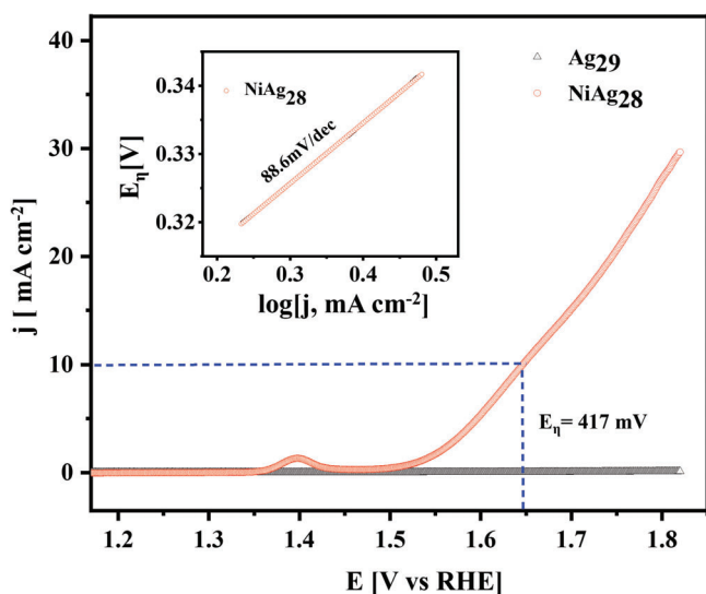
Figure 5. Electrochemical OER performance of NiAg 28 (red trace) compared to Ag 29 (black trace) in 1 M KOH electrolyte: Linear sweep voltammetry (LSV) curves (LSV were recorded at a sweep rate of 5 mV s -1 ), and the applied voltage was 417 mV for the NiAg 28 clusters when the current density was 10 mA cm -2 . The inset shows the Tafel plot of NiAg 28 NCs (with the potential E vs the potential of the RHE), which suggests a more favorable reaction kinetics.
